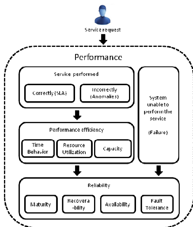
Figure 3. Context diagram for Cloud Computing performance measurement.
