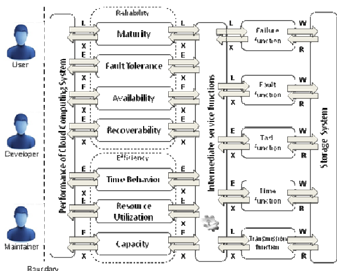
Figure 6. Detailed performance measurement model for CC.
