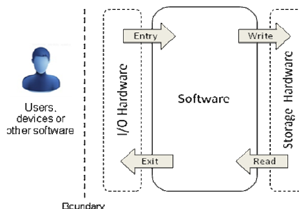
Figure 4. COSMIC model of generic software – adapted from Figure 12.4 of [12].
